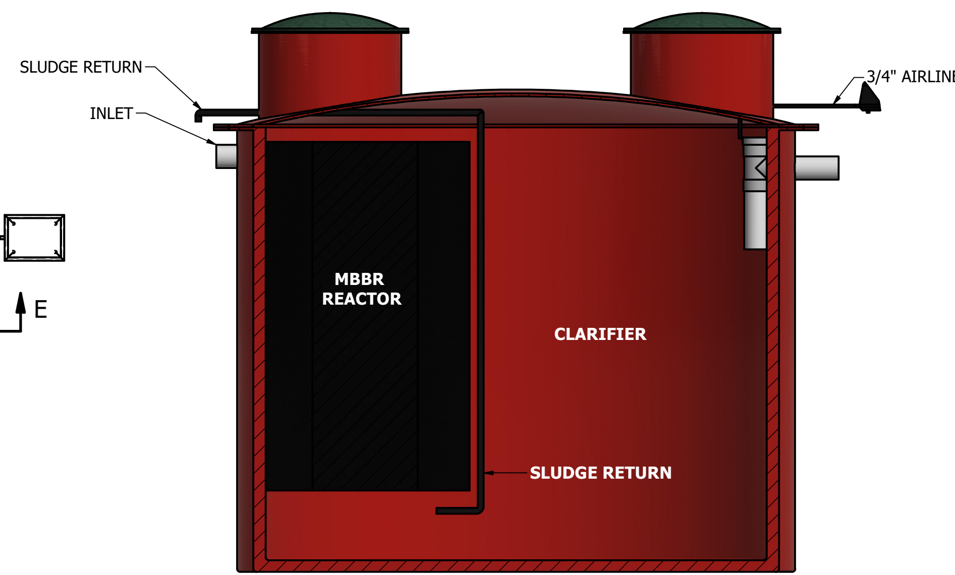
CUTAWAY
