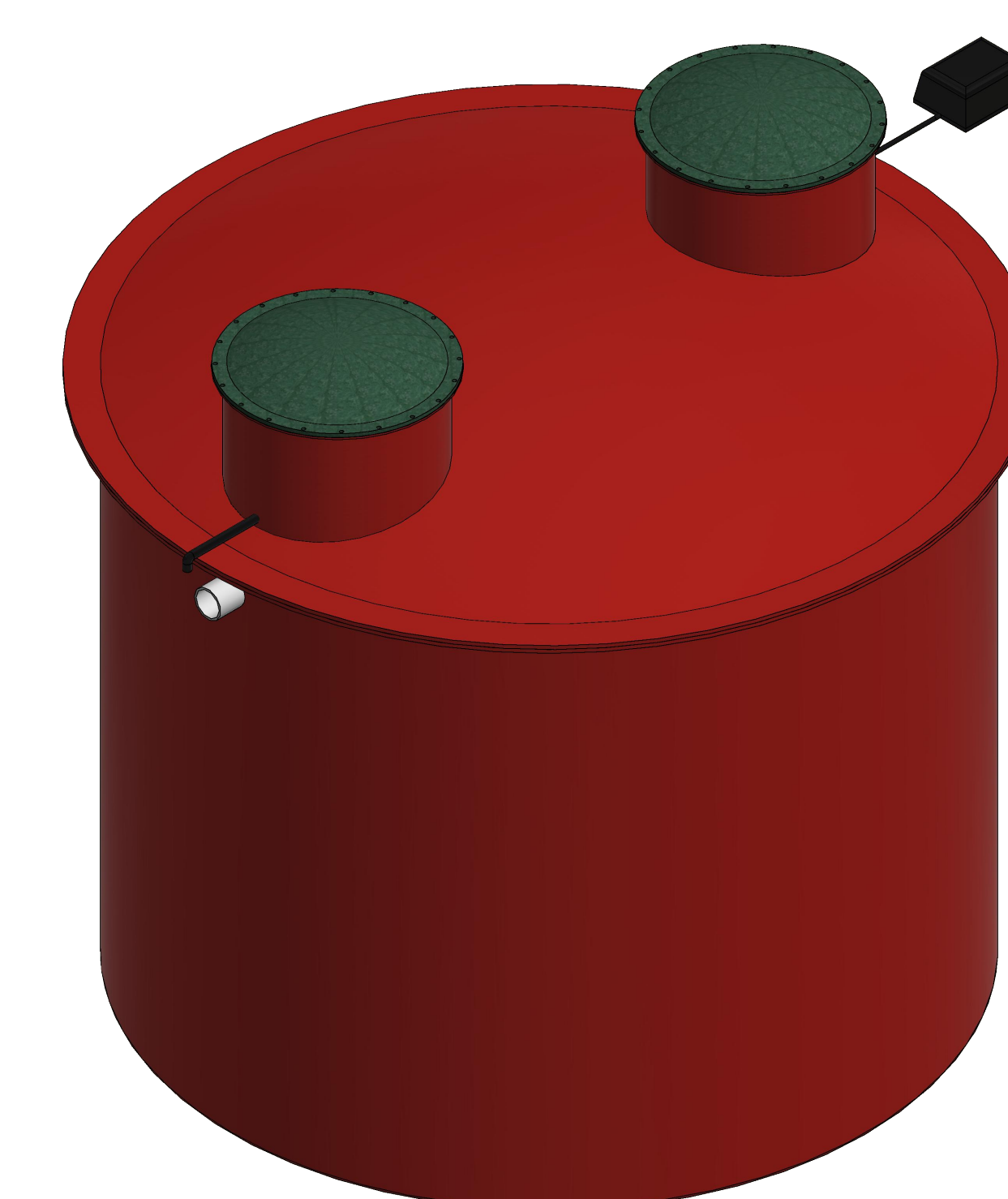
INLET SIDE
