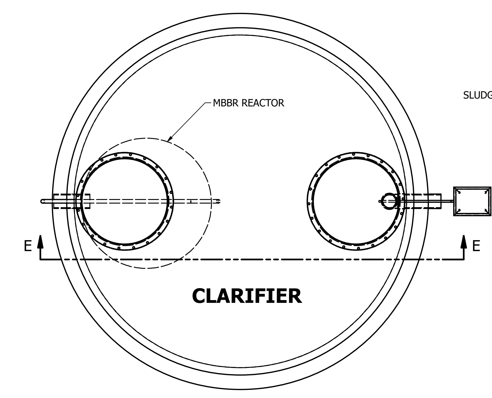
TOP VIEW
